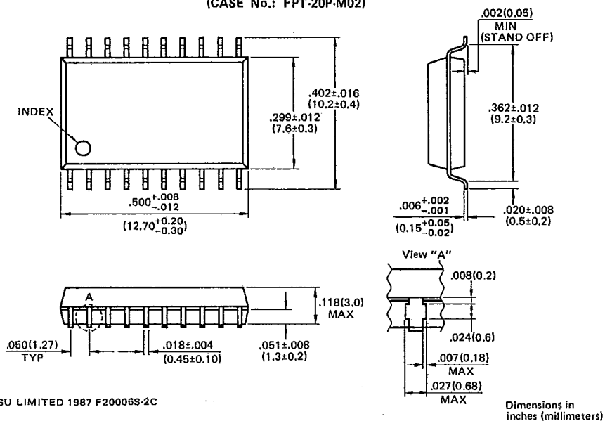
20-LEAD PLASTIC FLAT PACKAGE (CASE No.: FPT-20P-M02)
