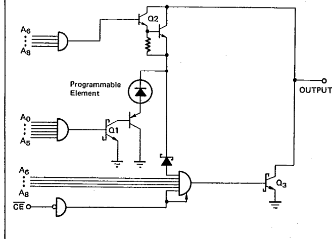
Fig. 25 — INTERNAL PROGRAMMING CIRCUIT
