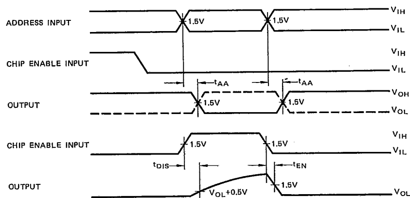
OPERATION TIMING DIAGRAM
