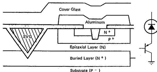
Fig. 24 — PROGRAMMED CELL (CROSS SECTION)
